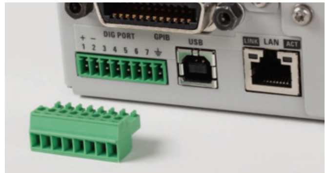
Figure 10. Digital control port on rear panel
