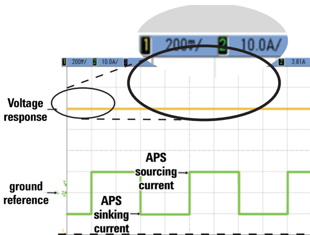
Figure 3 shows an example of an APS power supply smoothly pulsing back and forth from sinking current at -10 A to sourcing current at 10 A. Notice that the voltage level captured at high resolution on the top trace remains constant with no glitches.
