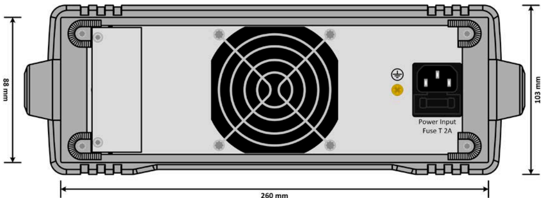
标配版的后视图 / Rear view of the standard configuration
